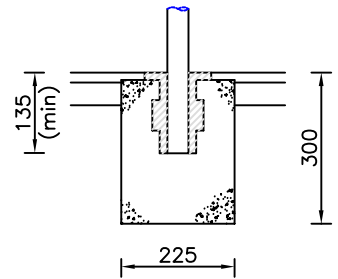
ALTERNATIVE SOCKET POST FOUNDATION
