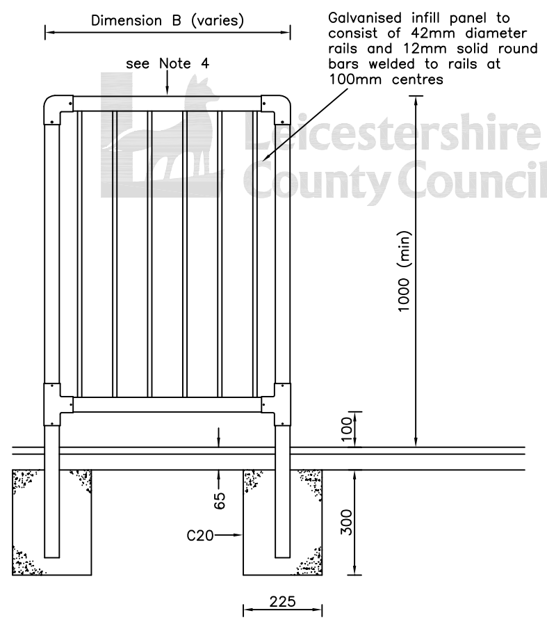
ELEVATION OF BARRIER PANEL
