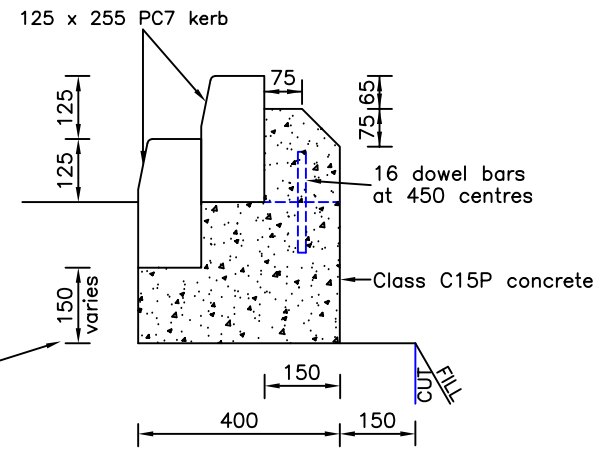
DOUBLE KERB - K19
