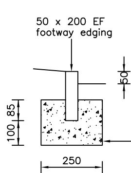
FOOTWAY EDGING EF 200
