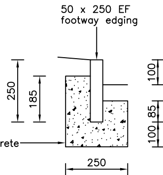
FOOTWAY EDGING EF 250
