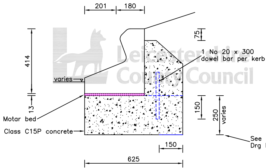
ELLIS - TRIEF SAFETY KERB - TYPE G ST/2A OR SIMILAR APPROVED
