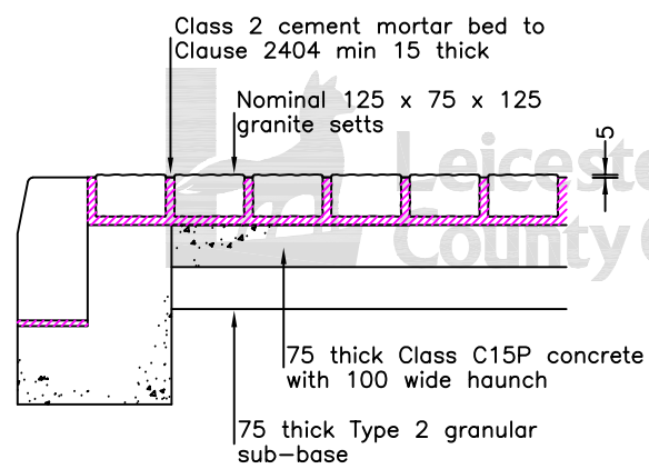
GRANITE SETTS TO ISLANDS, FOOTWAYS ETC
