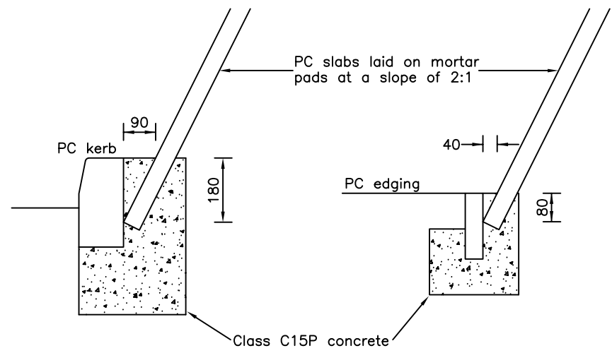
PC SLABS LAID ON EDGE
