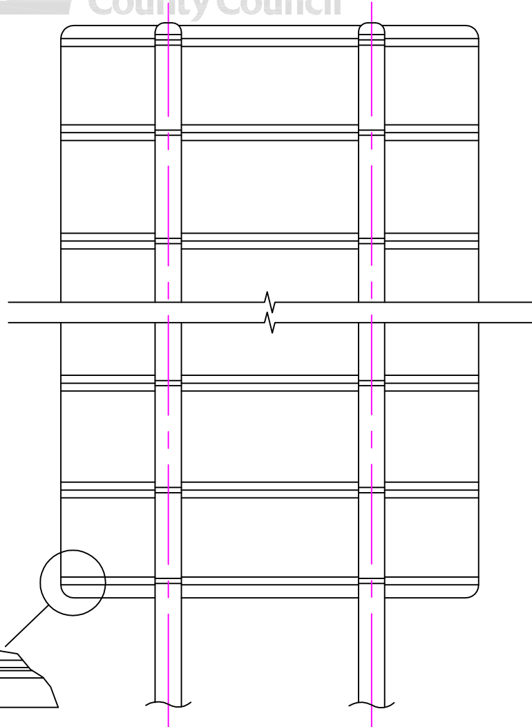
REAR VIEW OF SIGN
