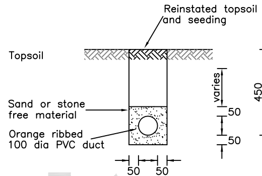
DUCT IN VERGE
