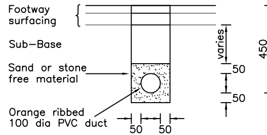
DUCT IN FOOTWAY
