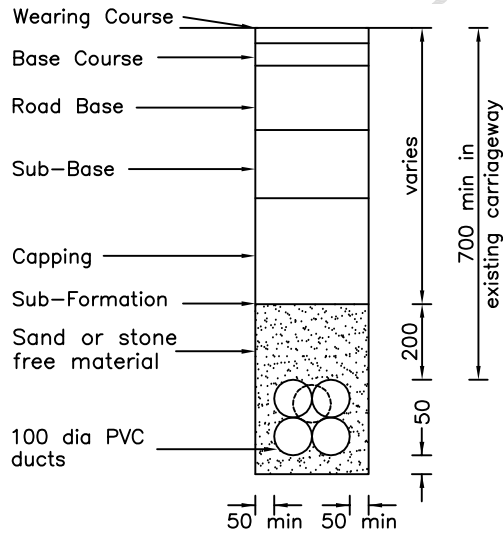
2, 3 OR 4 WAY DUCTS IN CARRIAGEWAY
