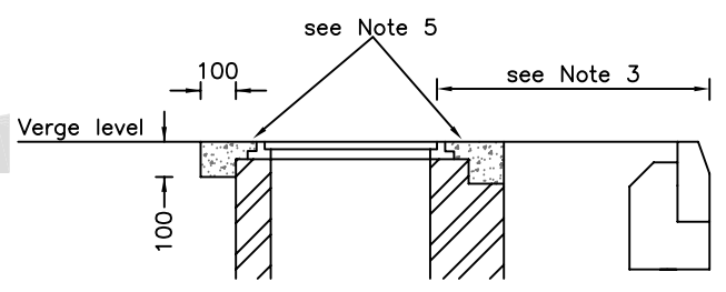
ALTERNATIVE DETAIL OF FIXING COVER FOR CHAMBER CONSTRUCTED IN VERGE
