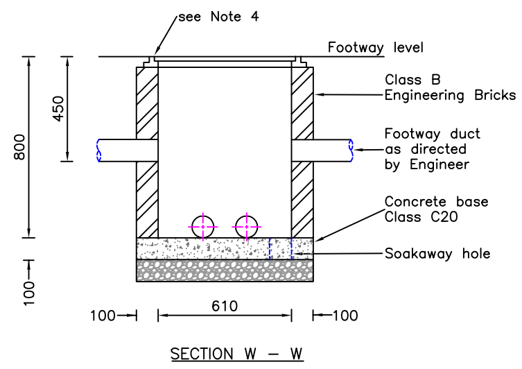
TYPE A - BRICKWORK CHAMBERS
