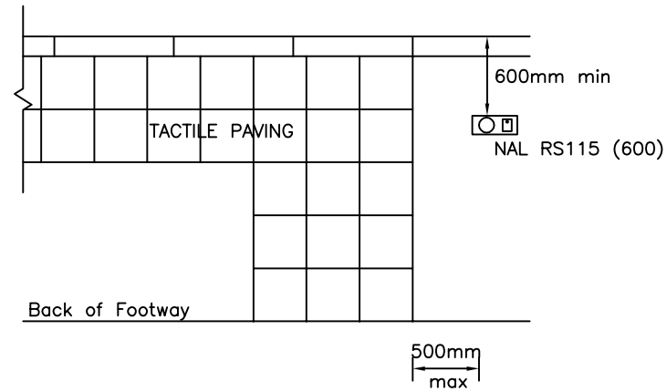
POLEBOX WITH SWANS NECK (CRANKED) POLE OR STUB POLE
