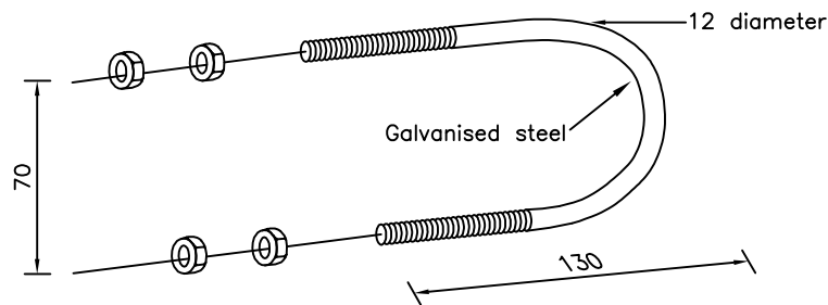
'D' CLAMP DETAIL
