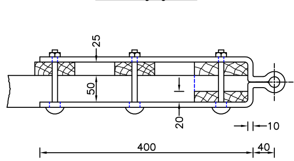
Detail of Joint between Top and Bottom Rails and Hanging Stile
