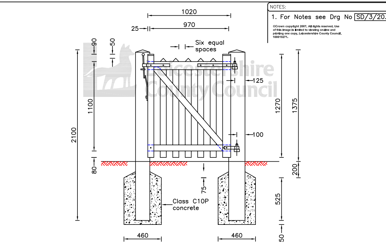
TIMBER WICKET GATE – TYPE 2
