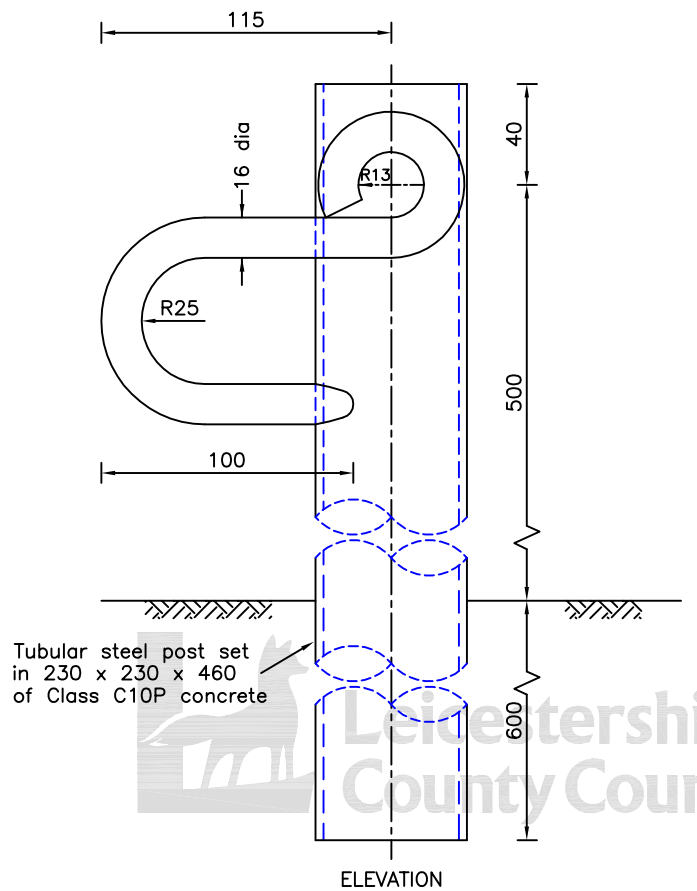
HOLDING BACK STOP POST FOR STEEL GATES
