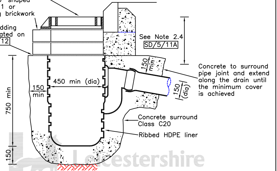
IN SITU CONCRETE GULLY CROSS SECTION
