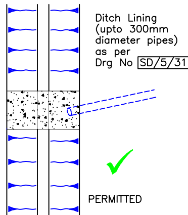
ARRANGEMENTS WHERE PIPES ENTER DITCH FROM THE SIDE (See Note 3)
