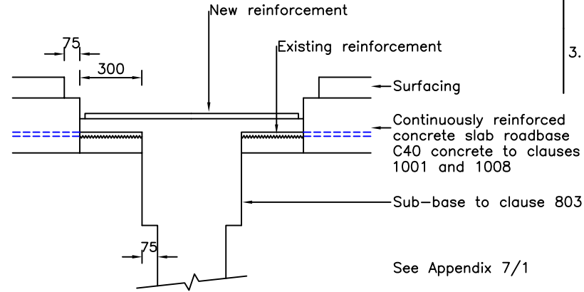
REINSTATEMENT OF CARRIAGEWAY WITH REINFORCED CONCRETE ROADBASE
