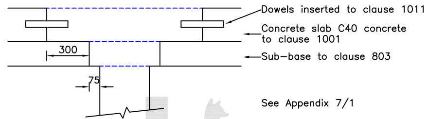
REINSTATEMENT OF CARRIAGEWAY WITH UNREINFORCED CONCRETE SLAB
