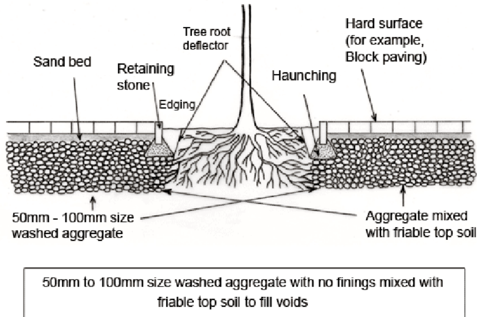
Figure L4 Planting in hard-surfaced areas
